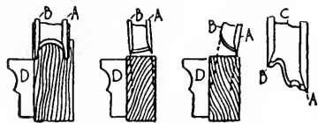
FIG. 74. ANGLES FOR SETTING FENCE, UNIVERSAL PLANE.
